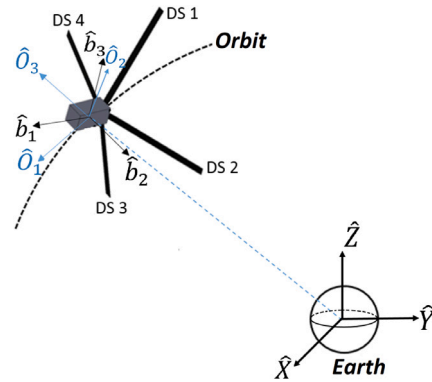
Fig. 2. Coordinate systems.
